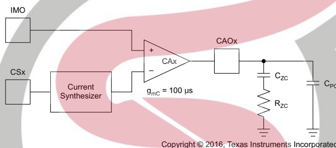
Figure 22. Current Error Amplifier With Type II Compensation
